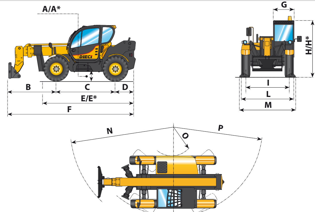
A* - E* - H* = Measurements referring to optional wheels
