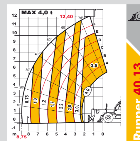
A* - E* - H* = Measurements referring to optional wheels
